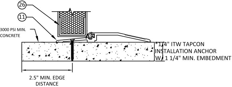
TYPE 2 -REPUBLIC THRESHOLD DETAIL (SILL) WITH FLUSH BOTTOM RAIL
