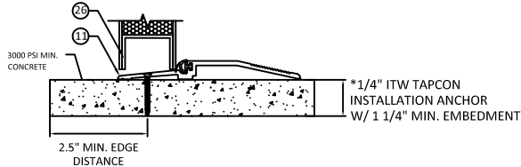
TYPE 2 REPUBLIC THRESHOLD DETAIL (SILL) WITH INVERTED BOTTOM RAIL
