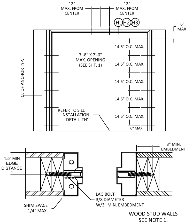
TYPE 1 EMA ANCHORS
